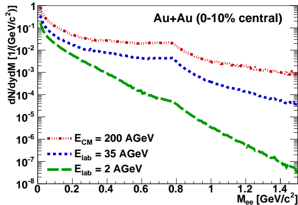
Fig. 2. Thermal dilepton invariant mass spectra dN/(dy dM) for central Au+Au collisions and the same energies as considered in Fig. 1. The results show the yield at mid-rapidity, |y_{ee}| < 0.5 .
