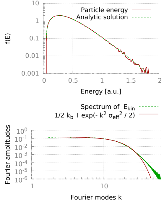
Figure 1: Upper panel: The quark-energy distribution from the kinetic Monte-Carlo simulation after a stationary state has been reached compared to the expected equilibrium-Boltzmann distribution \propto \exp(-E/T) . Lower panel: The Fourier spectrum of the mean field in comparison to the classical equipartition theorem, modified by an effective ultra-violet cutoff due to the finite extent of the interaction volume between particle creation and annihilation processes.
