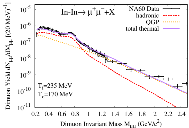
Figure 1: (Color online) Excess dimuon invariant-mass spectra in In-In ( \sqrt{s_{NN}} = 17.3 GeV) collisions at the SPS. Theoretical calculations (solid line), composed of hadronic radiation (using in-medium \rho and \omega spectral functions and multi-pion annihilation with chiral mixing, dashed line) and QGP radiation (using a lattice-QCD inspired rate, dotted line) are compared to NA60 data [49, 12].
