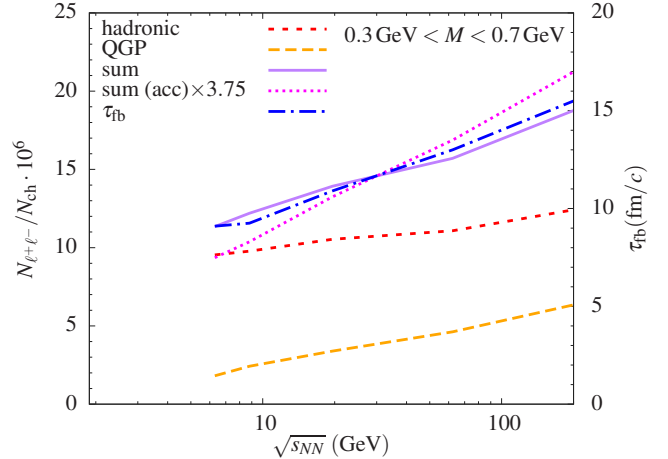
Figure 3: (Color online) Excitation function of low-mass thermal dilepton radiation (“excess spectra”) in 0-10% central AA collisions ( A \simeq 200 ), integrated over the mass range M = 0.3 GeV- 0.7 GeV, for QGP (dashed line) and in-medium hadronic (short-dashed line) emission and their sum (solid line). The underlying fireball lifetime (dot-dashed line) is given by the right vertical scale.
