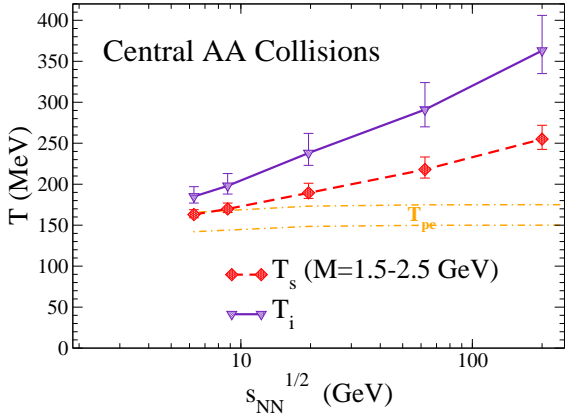
Figure 2: (Color online) Excitation function of the inverse-slope parameter, T_s , from intermediate-mass dilepton spectra ( M = 1.5 - 2.5 GeV, diamonds connected with dashed line) and initial temperature T_0 (triangles connected with solid line) in central heavy-ion collisions ( A \simeq 200 ). The error bars on T_s and T_0 correspond to a variation in the initial longitudinal fireball size, z_0 , by \pm 30\% around the central values quoted in Table 1. The hatched area schematically indicates the pseudo-critical temperature regime at vanishing (and small) chemical potential as extracted from various quantities computed in lattice QCD [15].
