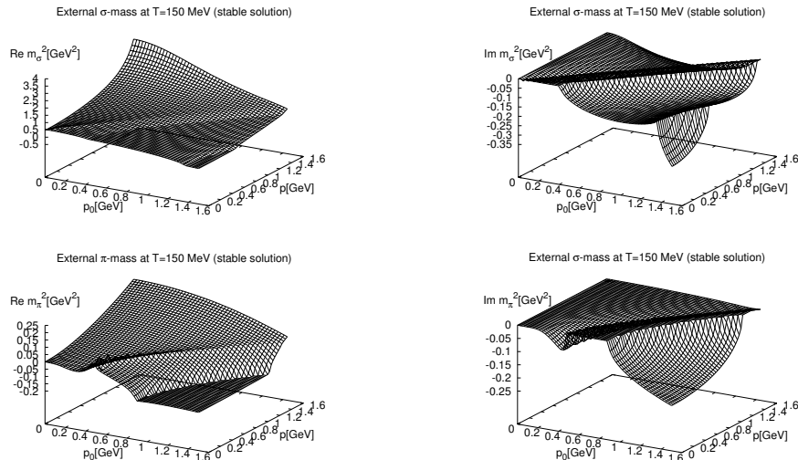
Figure 5. The effective external masses at a temperature of 150MeV. The effective external \pi -mass indeed vanishes at p_0 = \vec{p} = 0 as predicted from Goldstone's theorem. The spectral function of the \sigma -meson shows that at high temperatures its strength becomes more peaked and the maximum shifted to lower momenta than at T = 0 .
